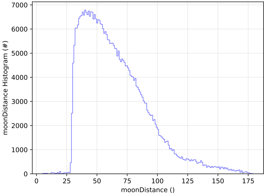
too_elab_2yr_r32_d2_ugrizy_v3.4_10yrs WFD y band: moonDistance Histogram
