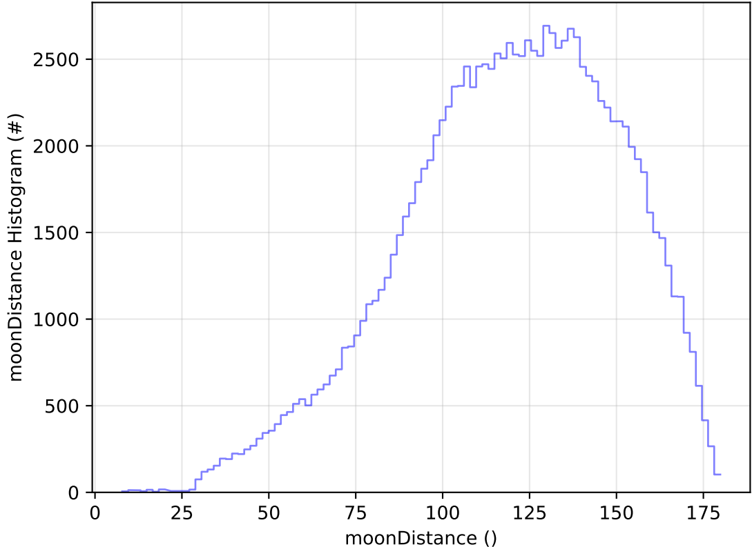
too_elab_2yr_r32_d2_ugrizy_v3.4_10yrs WFD u band: moonDistance Histogram
