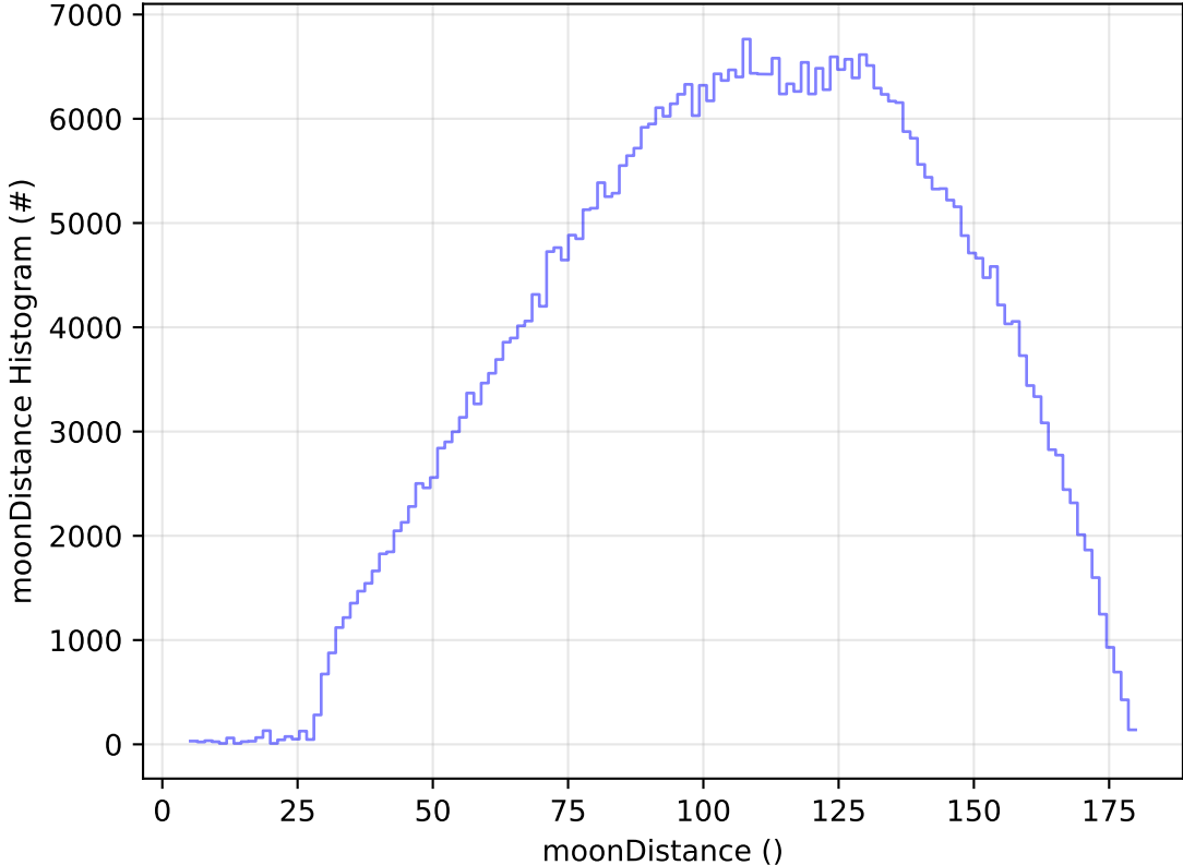
too_elab_2yr_r32_d2_ugrizy_v3.4_10yrs WFD r band: moonDistance Histogram
