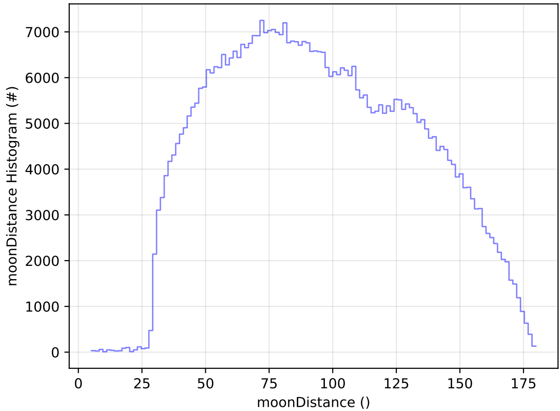
too_elab_2yr_r32_d2_ugrizy_v3.4_10yrs WFD i band: moonDistance Histogram
