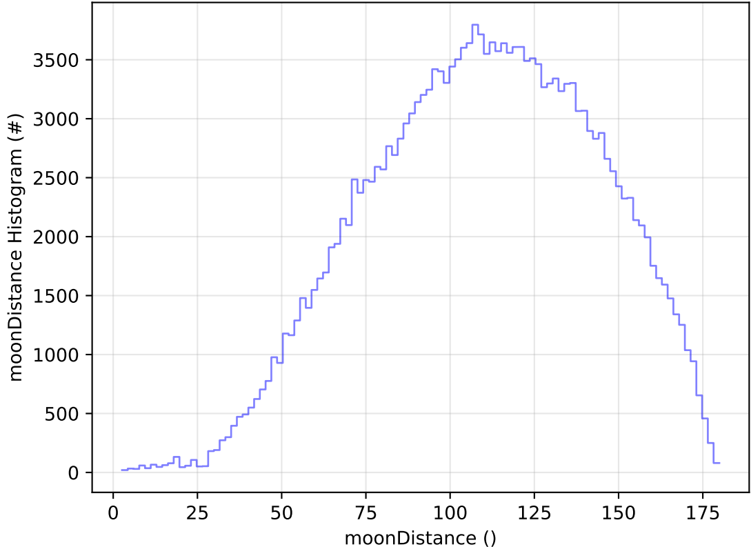
too_elab_2yr_r32_d2_ugrizy_v3.4_10yrs WFD g band: moonDistance Histogram
