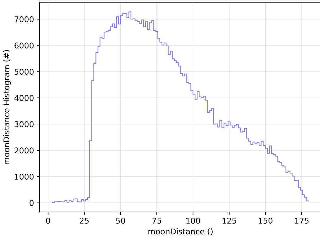
too_elab_2yr_r32_d2_ugrizy_v3.4_10yrs All sky z band: moonDistance Histogram
