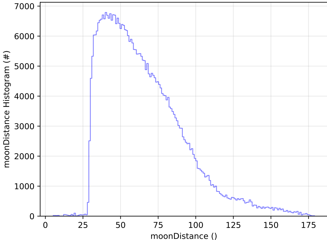
too_elab_2yr_r32_d2_ugrizy_v3.4_10yrs All sky y band: moonDistance Histogram
