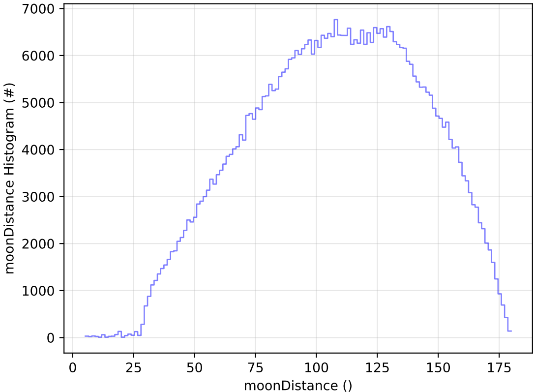
too_elab_2yr_r32_d2_ugrizy_v3.4_10yrs All sky r band: moonDistance Histogram
