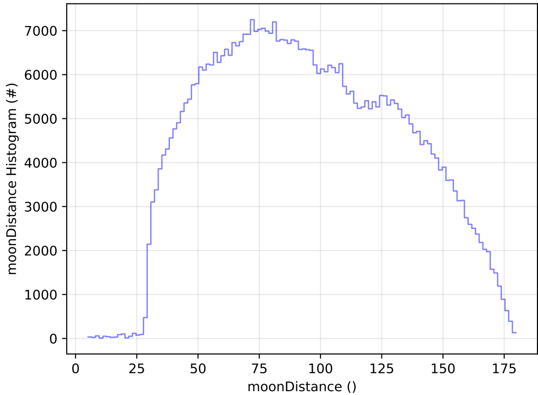
too_elab_2yr_r32_d2_ugrizy_v3.4_10yrs All sky i band: moonDistance Histogram
