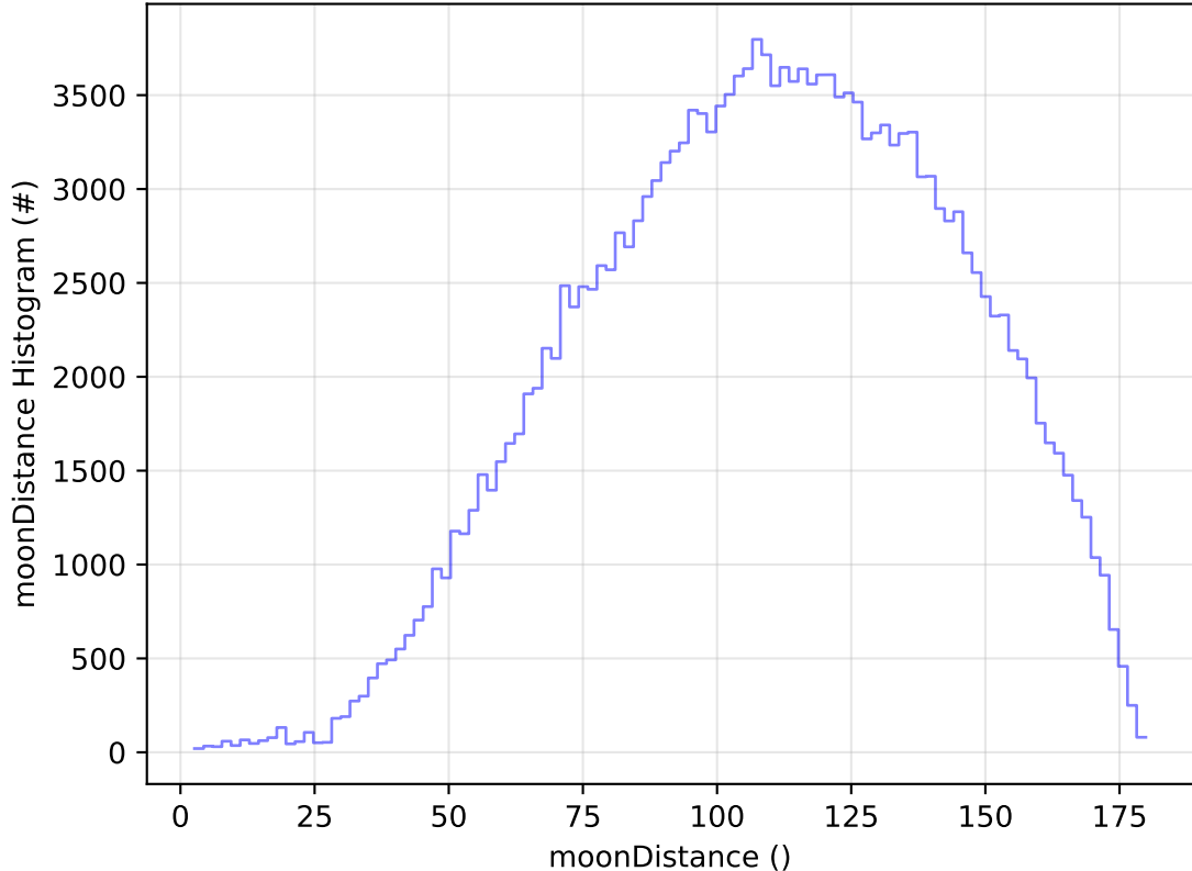
too_elab_2yr_r32_d2_ugrizy_v3.4_10yrs All sky g band: moonDistance Histogram
