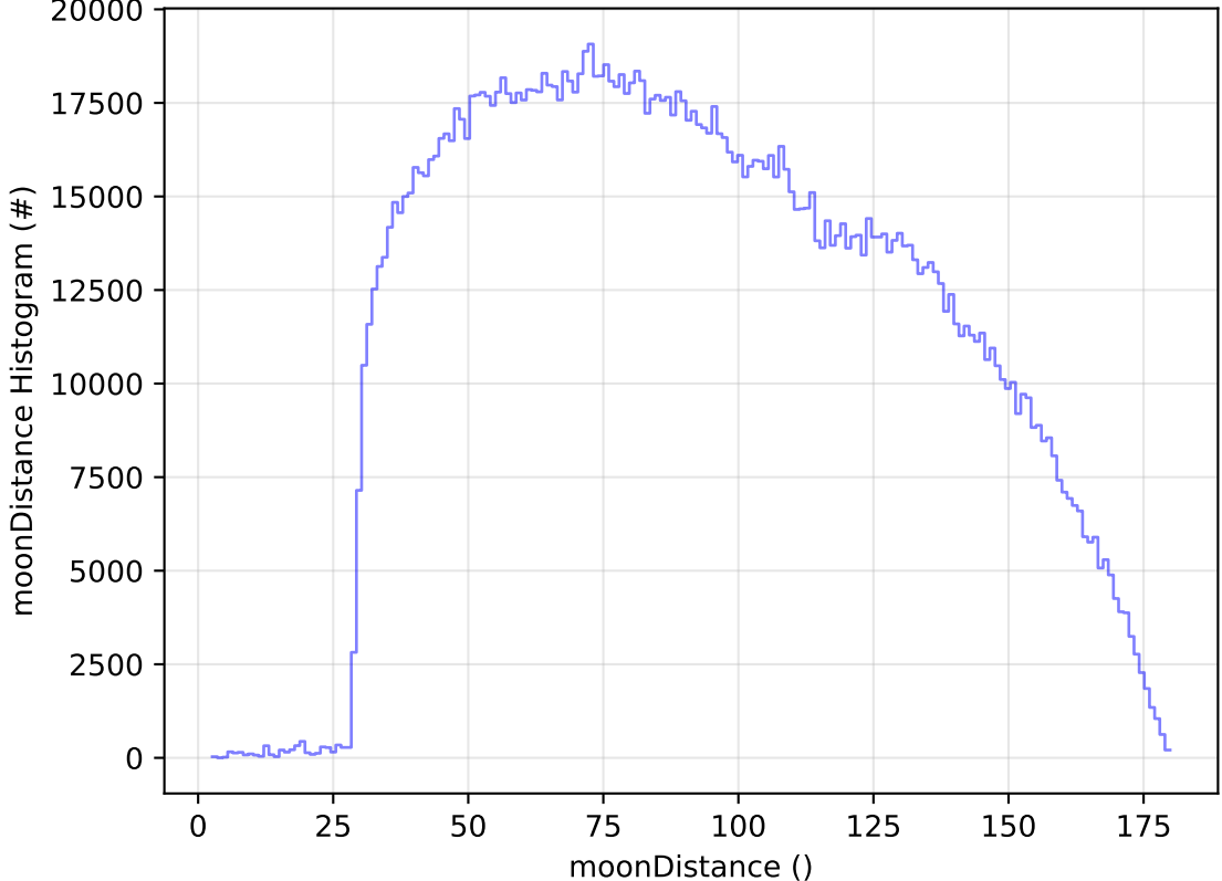
too_elab_2yr_r32_d2_ugrizy_v3.4_10yrs All sky all bands: moonDistance Histogram
