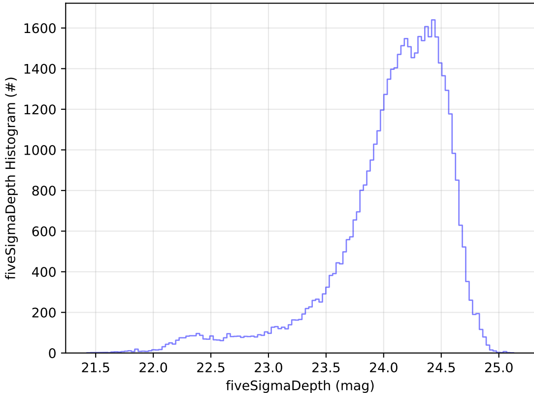
too_elab_2yr_r32_d2_ugrizy_v3.4_10yrs Yr 1 r band: fiveSigmaDepth Histogram
