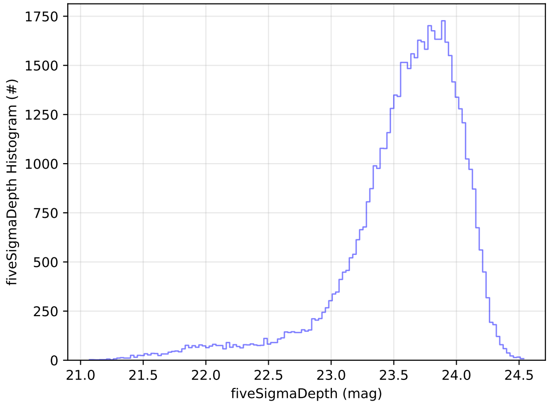
too_elab_2yr_r32_d2_ugrizy_v3.4_10yrs Yr 1 i band: fiveSigmaDepth Histogram
