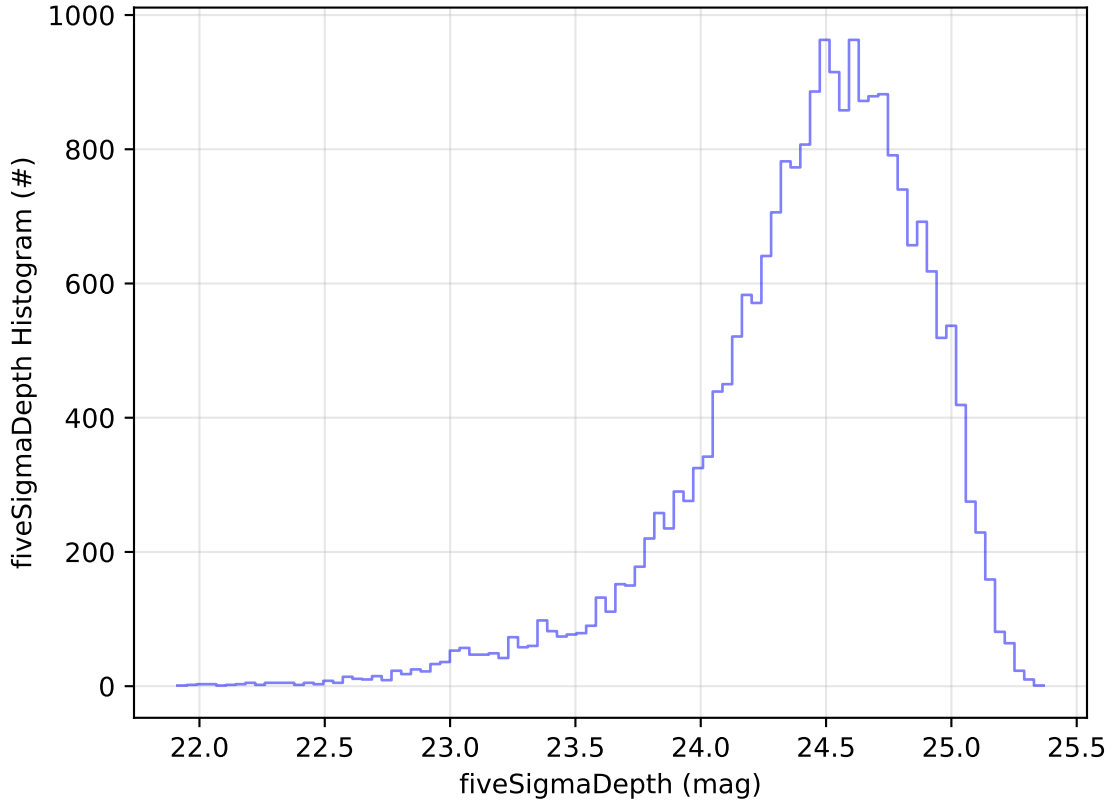
too_elab_2yr_r32_d2_ugrizy_v3.4_10yrs Yr 1 g band: fiveSigmaDepth Histogram
