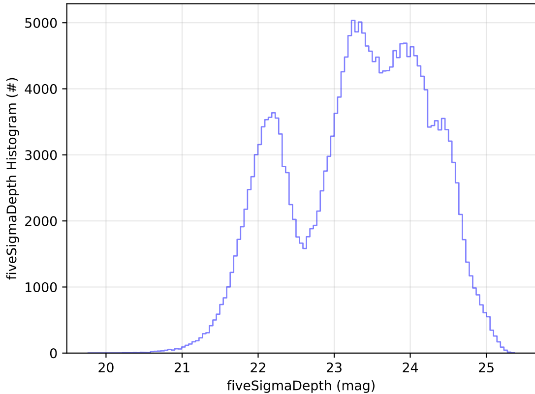
too_elab_2yr_r32_d2_ugrizy_v3.4_10yrs Yr 1 all bands: fiveSigmaDepth Histogram
