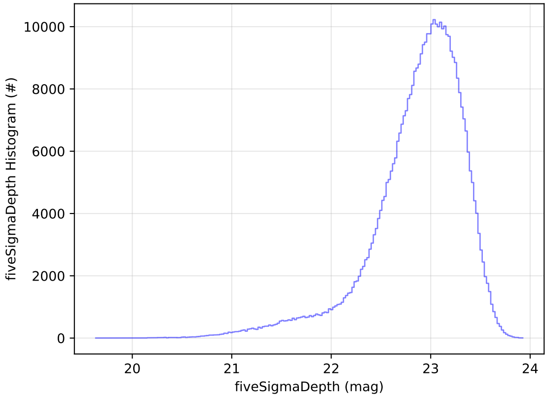
too_elab_2yr_r32_d2_ugrizy_v3.4_10yrs WFD z band: fiveSigmaDepth Histogram
