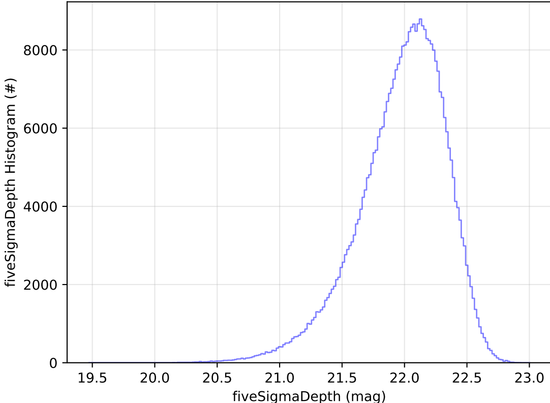
too_elab_2yr_r32_d2_ugrizy_v3.4_10yrs WFD y band: fiveSigmaDepth Histogram
