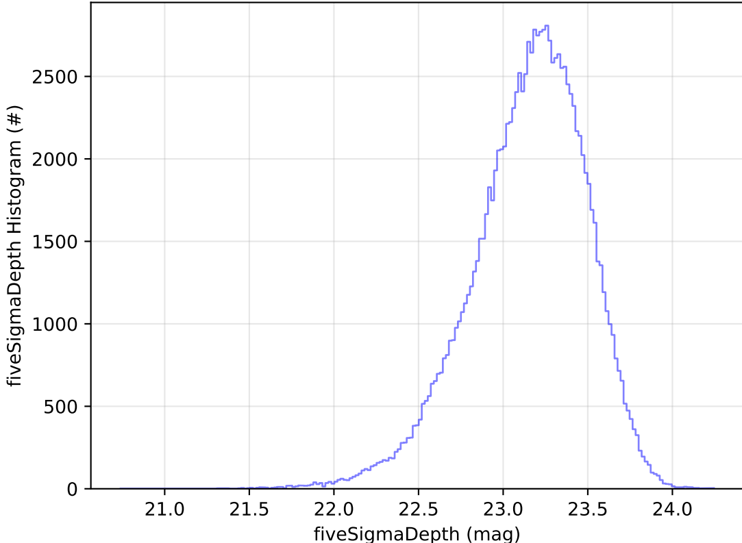
too_elab_2yr_r32_d2_ugrizy_v3.4_10yrs WFD u band: fiveSigmaDepth Histogram
