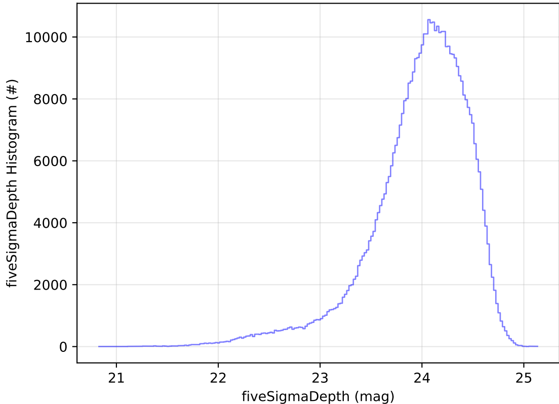
too_elab_2yr_r32_d2_ugrizy_v3.4_10yrs WFD r band: fiveSigmaDepth Histogram
