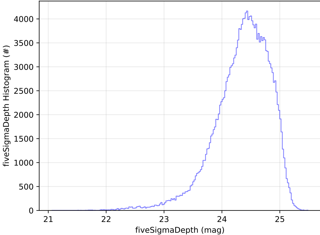
too_elab_2yr_r32_d2_ugrizy_v3.4_10yrs WFD g band: fiveSigmaDepth Histogram
