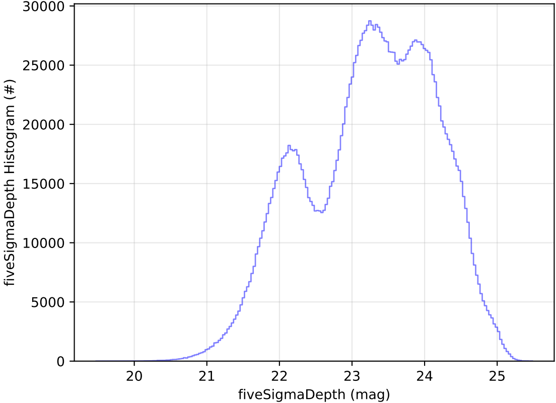
too_elab_2yr_r32_d2_ugrizy_v3.4_10yrs WFD all bands: fiveSigmaDepth Histogram
