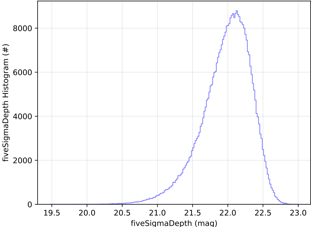
too_elab_2yr_r32_d2_ugrizy_v3.4_10yrs All sky y band: fiveSigmaDepth Histogram
