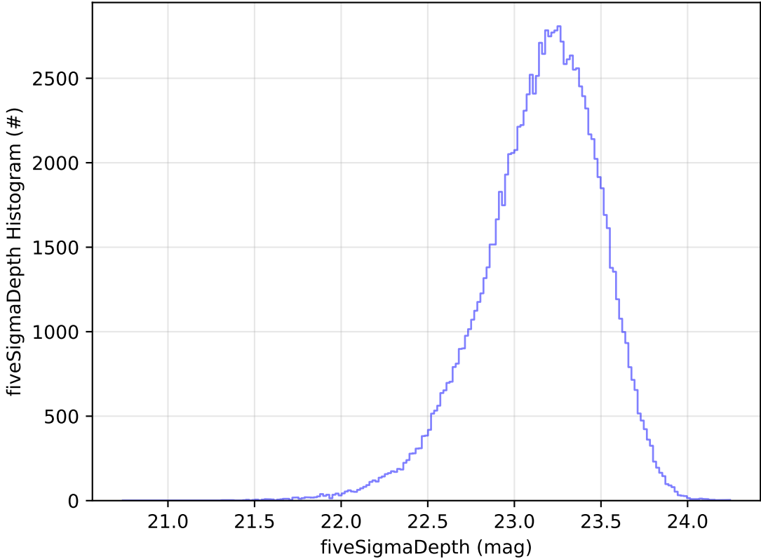
too_elab_2yr_r32_d2_ugrizy_v3.4_10yrs All sky u band: fiveSigmaDepth Histogram
