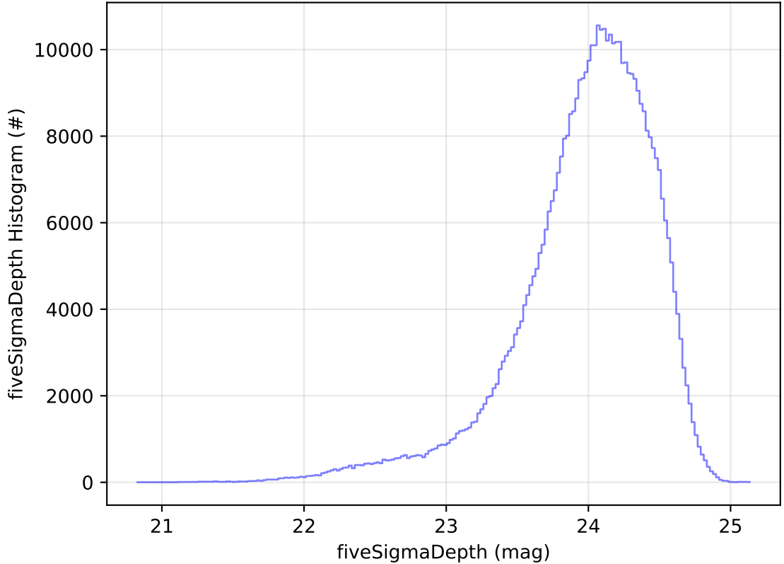
too_elab_2yr_r32_d2_ugrizy_v3.4_10yrs All sky r band: fiveSigmaDepth Histogram
