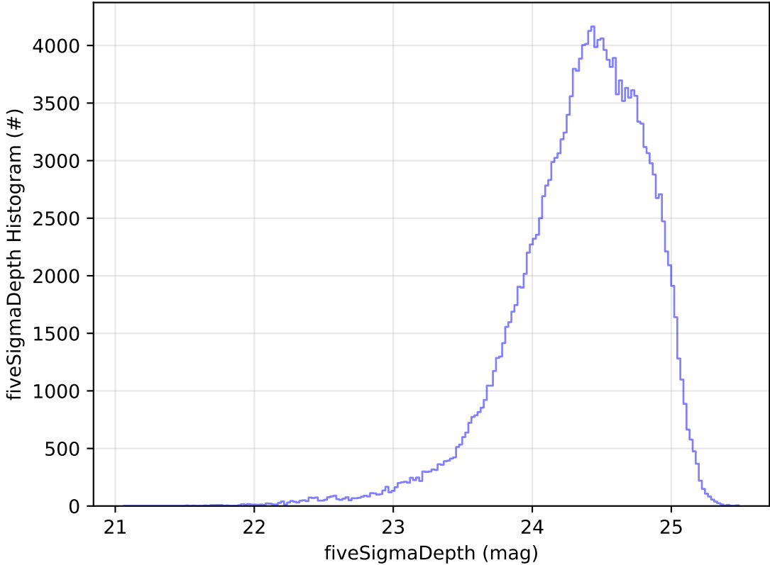
too_elab_2yr_r32_d2_ugrizy_v3.4_10yrs All sky g band: fiveSigmaDepth Histogram
