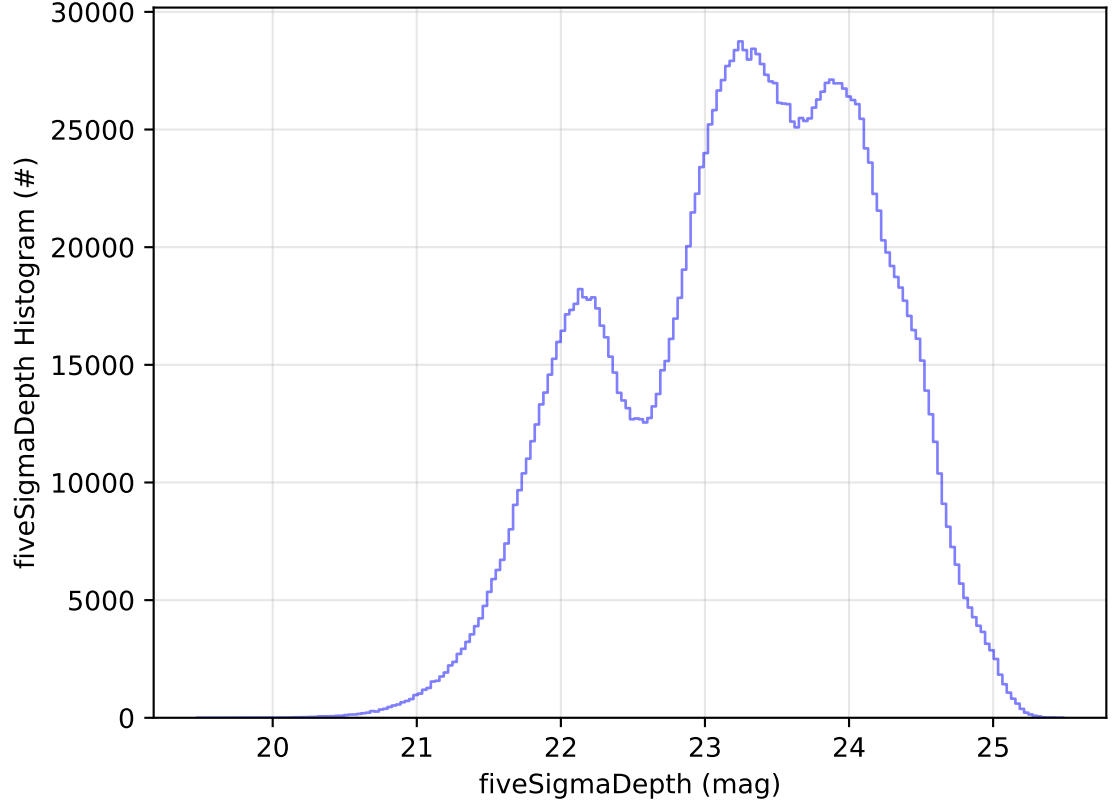
too_elab_2yr_r32_d2_ugrizy_v3.4_10yrs All sky all bands: fiveSigmaDepth Histogram
