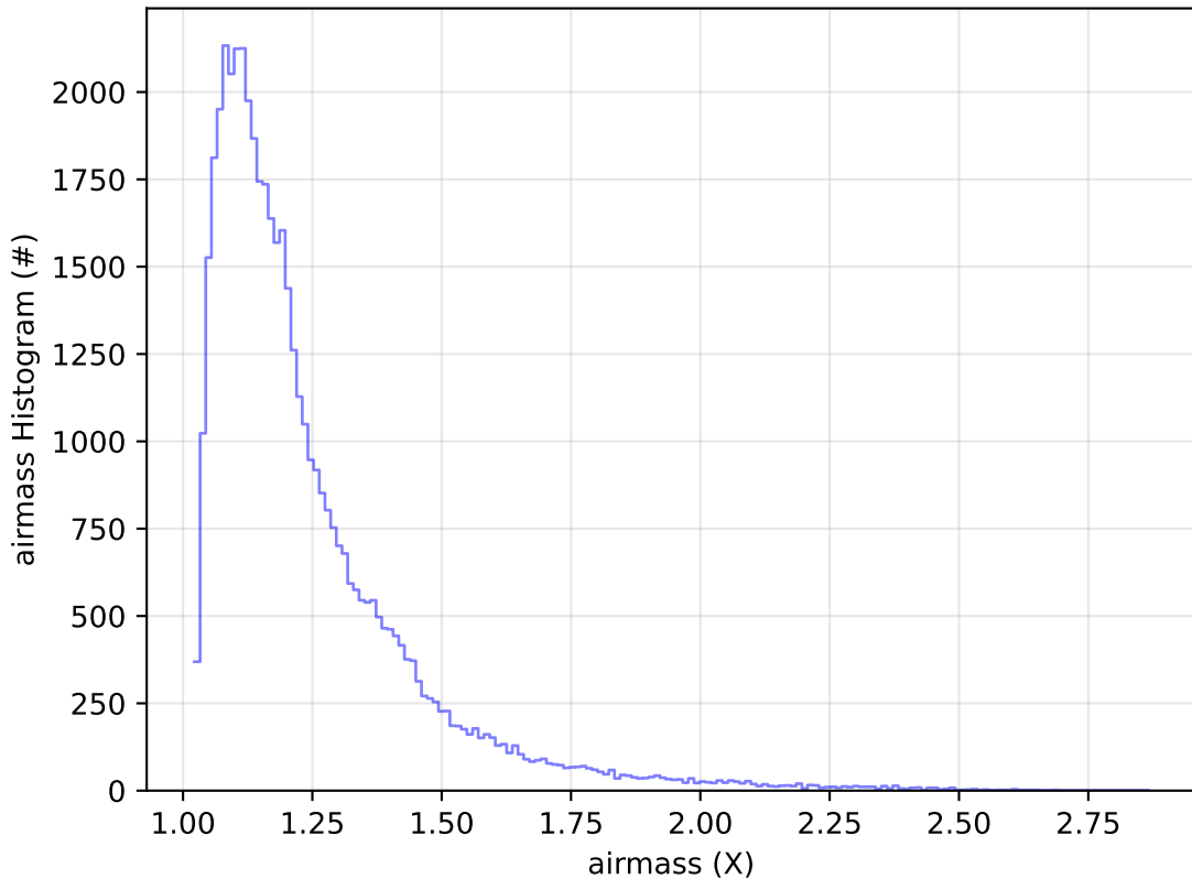
too_elab_2yr_r32_d2_ugrizy_v3.4_10yrs Yr 1 y band: airmass Histogram
