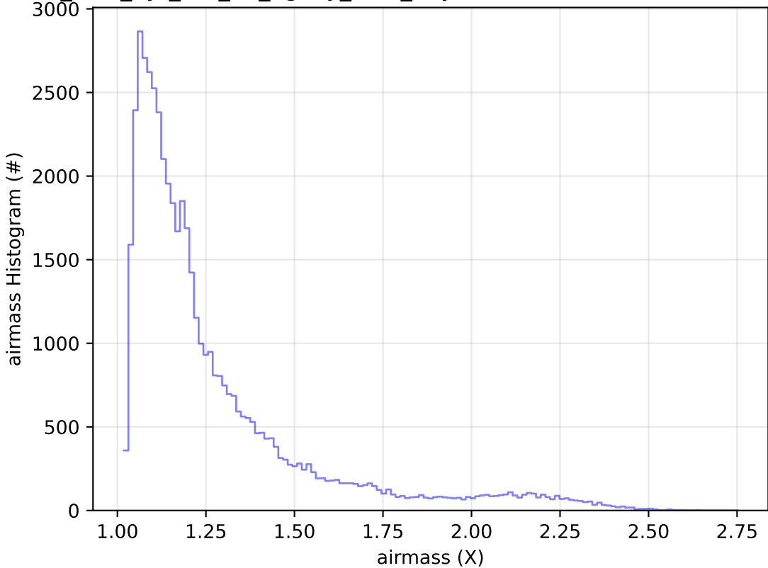
too_elab_2yr_r32_d2_ugrizy_v3.4_10yrs Yr 1 r band: airmass Histogram
