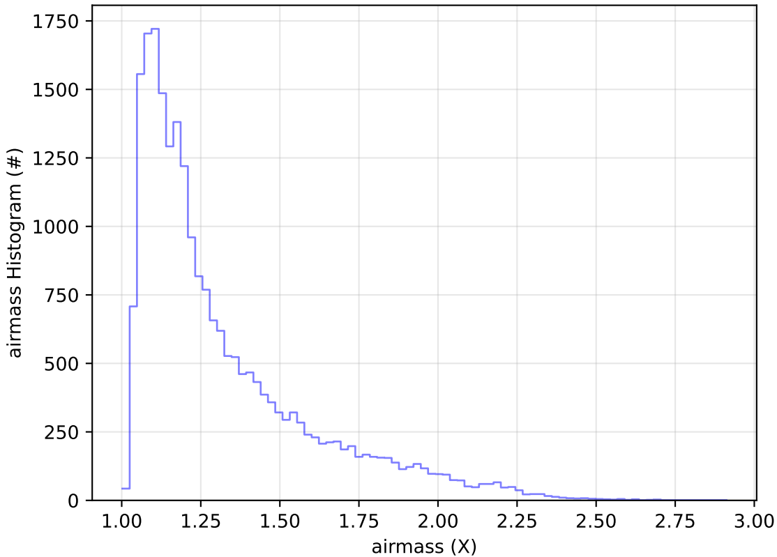
too_elab_2yr_r32_d2_ugrizy_v3.4_10yrs Yr 1 g band: airmass Histogram
