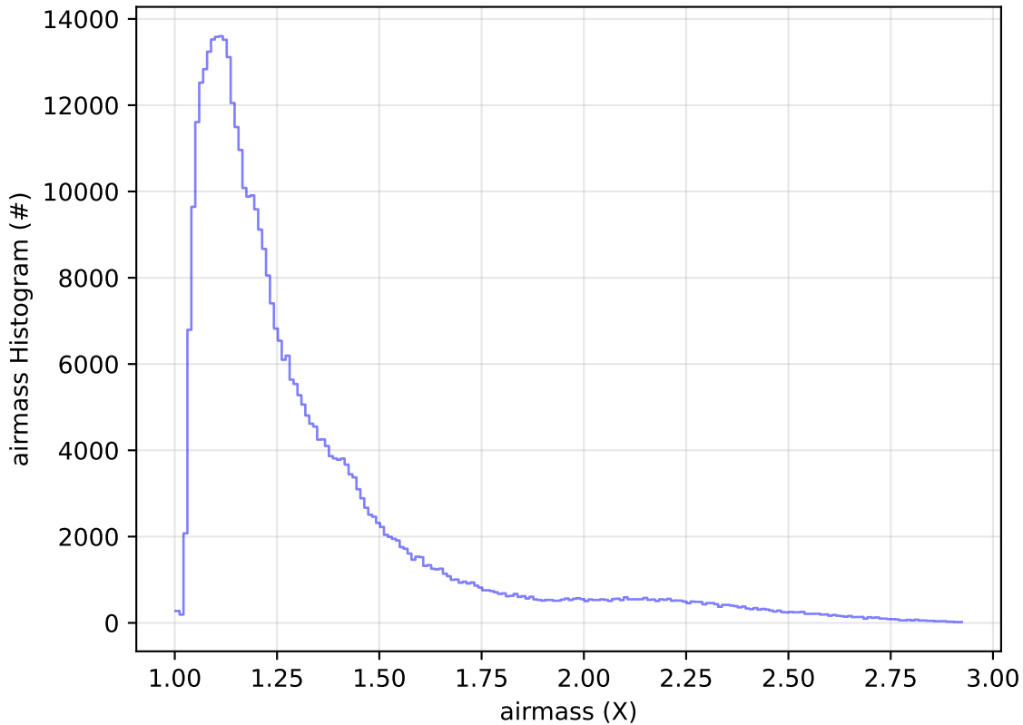
too_elab_2yr_r32_d2_ugrizy_v3.4_10yrs WFD z band: airmass Histogram
