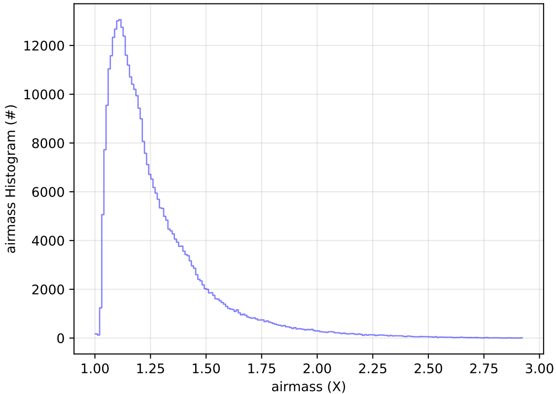
too_elab_2yr_r32_d2_ugrizy_v3.4_10yrs WFD y band: airmass Histogram
