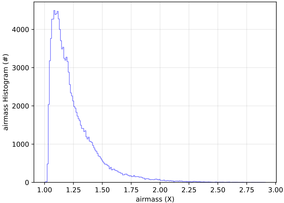
too_elab_2yr_r32_d2_ugrizy_v3.4_10yrs WFD u band: airmass Histogram
