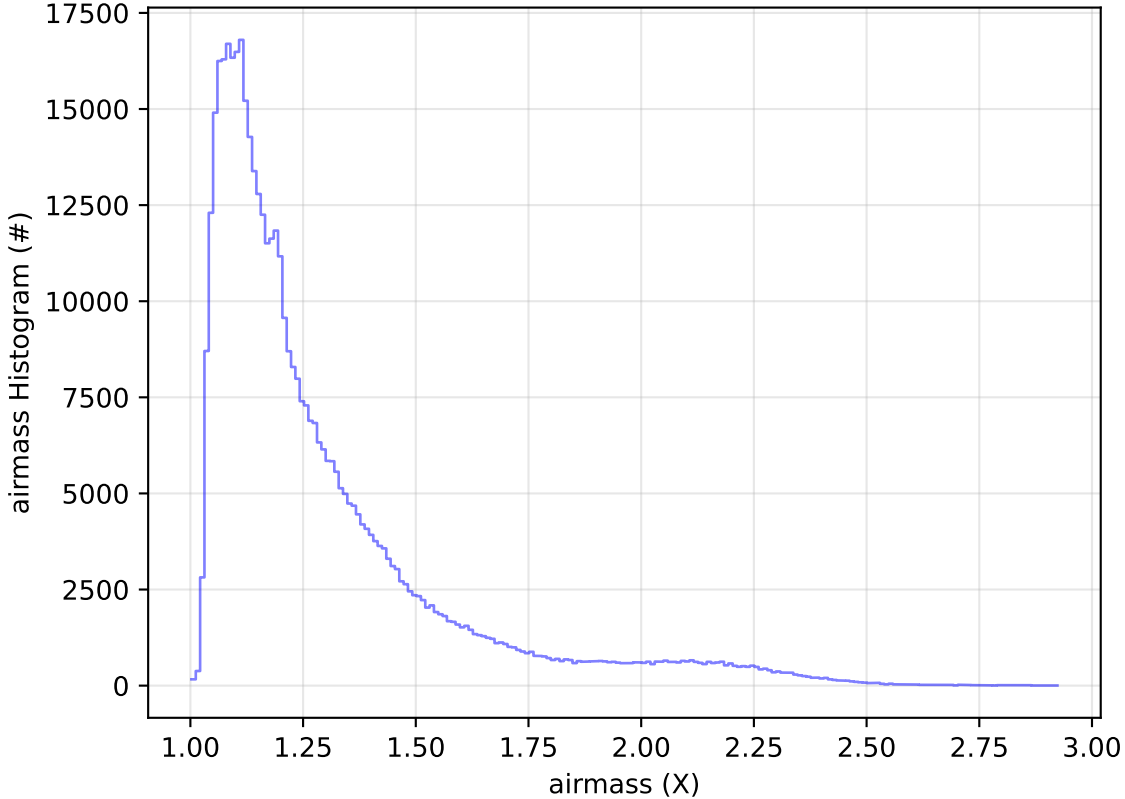
too_elab_2yr_r32_d2_ugrizy_v3.4_10yrs WFD r band: airmass Histogram
