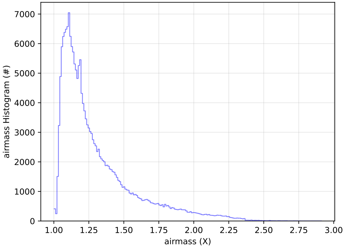
too_elab_2yr_r32_d2_ugrizy_v3.4_10yrs WFD g band: airmass Histogram
