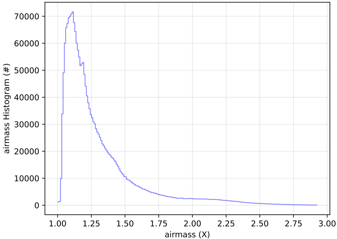
too_elab_2yr_r32_d2_ugrizy_v3.4_10yrs WFD all bands: airmass Histogram
