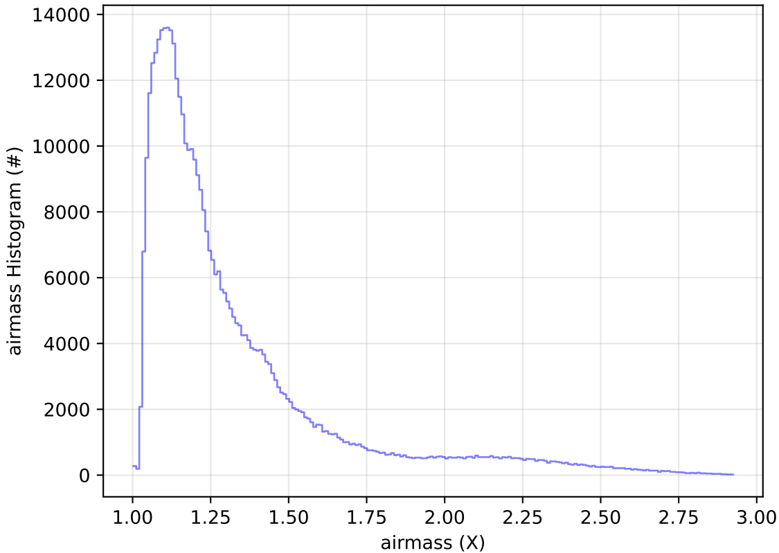
too_elab_2yr_r32_d2_ugrizy_v3.4_10yrs All sky z band: airmass Histogram
