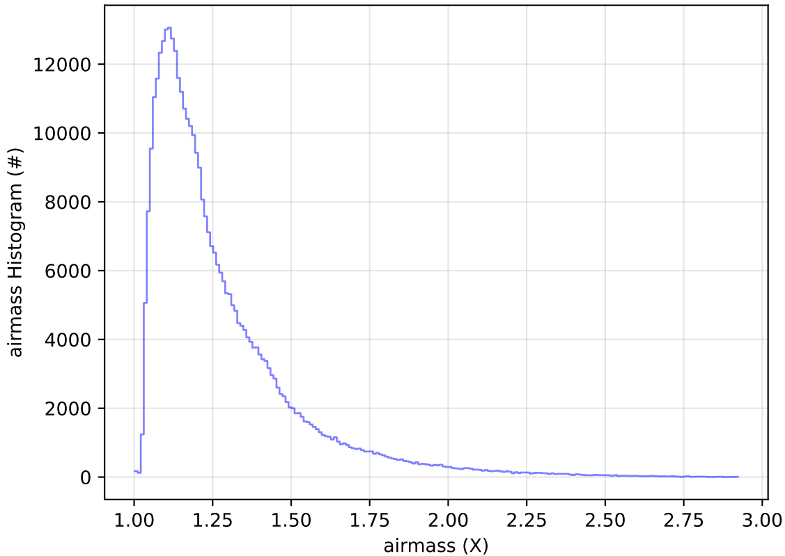
too_elab_2yr_r32_d2_ugrizy_v3.4_10yrs All sky y band: airmass Histogram
