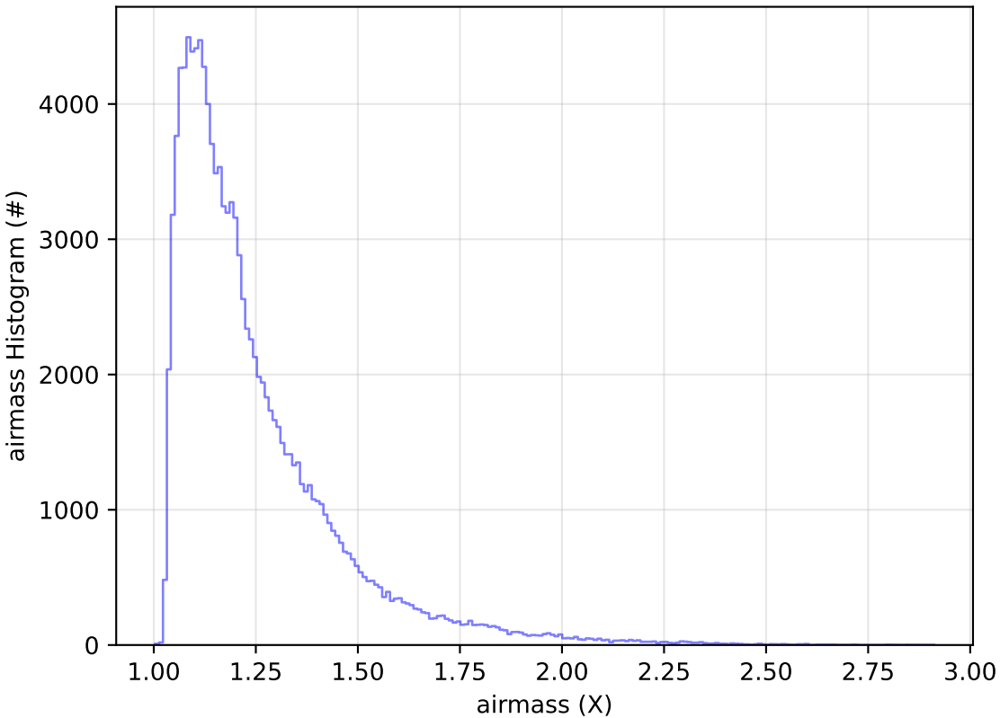
too_elab_2yr_r32_d2_ugrizy_v3.4_10yrs All sky u band: airmass Histogram
