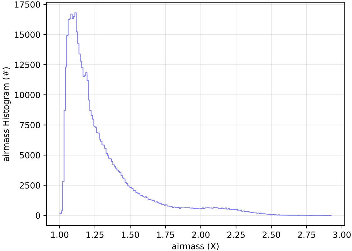
too_elab_2yr_r32_d2_ugrizy_v3.4_10yrs All sky r band: airmass Histogram
