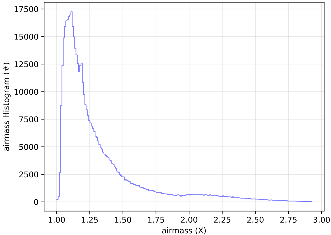
too_elab_2yr_r32_d2_ugrizy_v3.4_10yrs All sky i band: airmass Histogram
