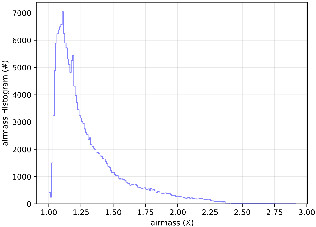
too_elab_2yr_r32_d2_ugrizy_v3.4_10yrs All sky g band: airmass Histogram
