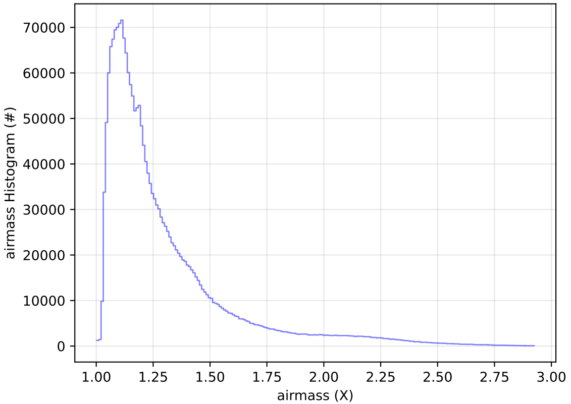
too_elab_2yr_r32_d2_ugrizy_v3.4_10yrs All sky all bands: airmass Histogram
