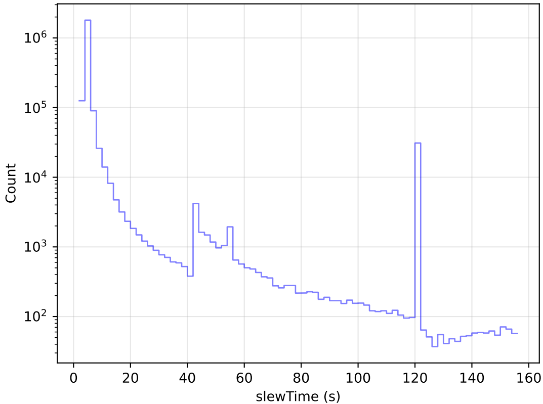
too_elab_2yr_r32_d2_ugrizy_v3.4_10yrs All visits: Slew Time Histogram
