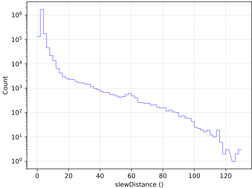
too_elab_2yr_r32_d2_ugrizy_v3.4_10yrs All visits: Slew Distance Histogram
