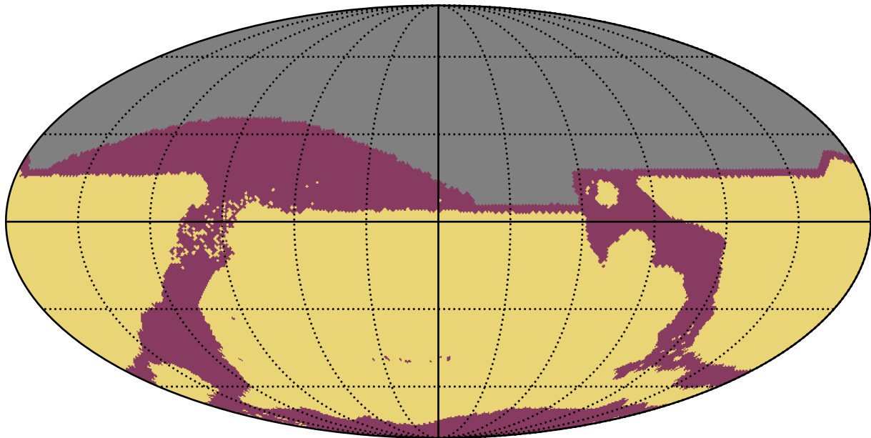
too_elab_2yr_r32_d2_ugrizy_v3.4_10yrs All sky: RapidRevisits
