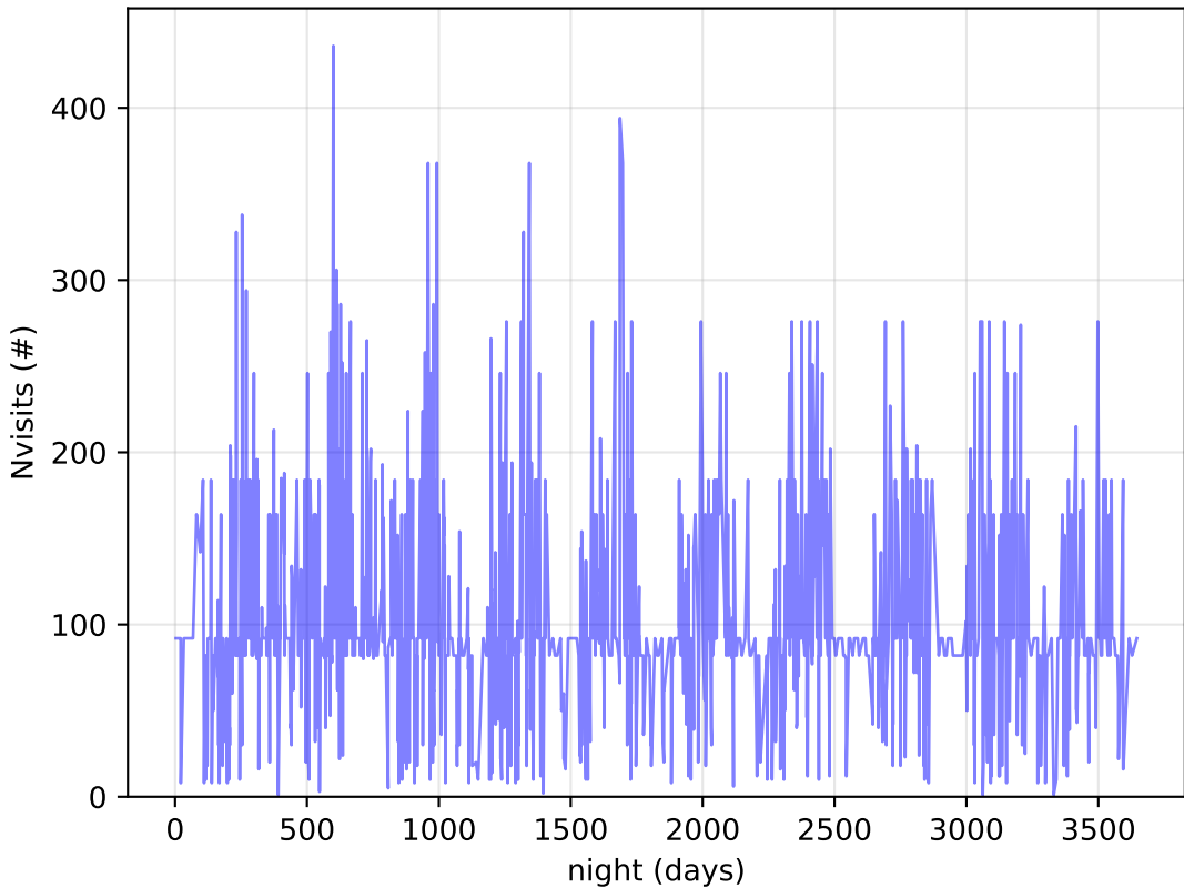
too_elab_2yr_r32_d2_ugrizy_v3.4_10yrs DDF: Nvisits
