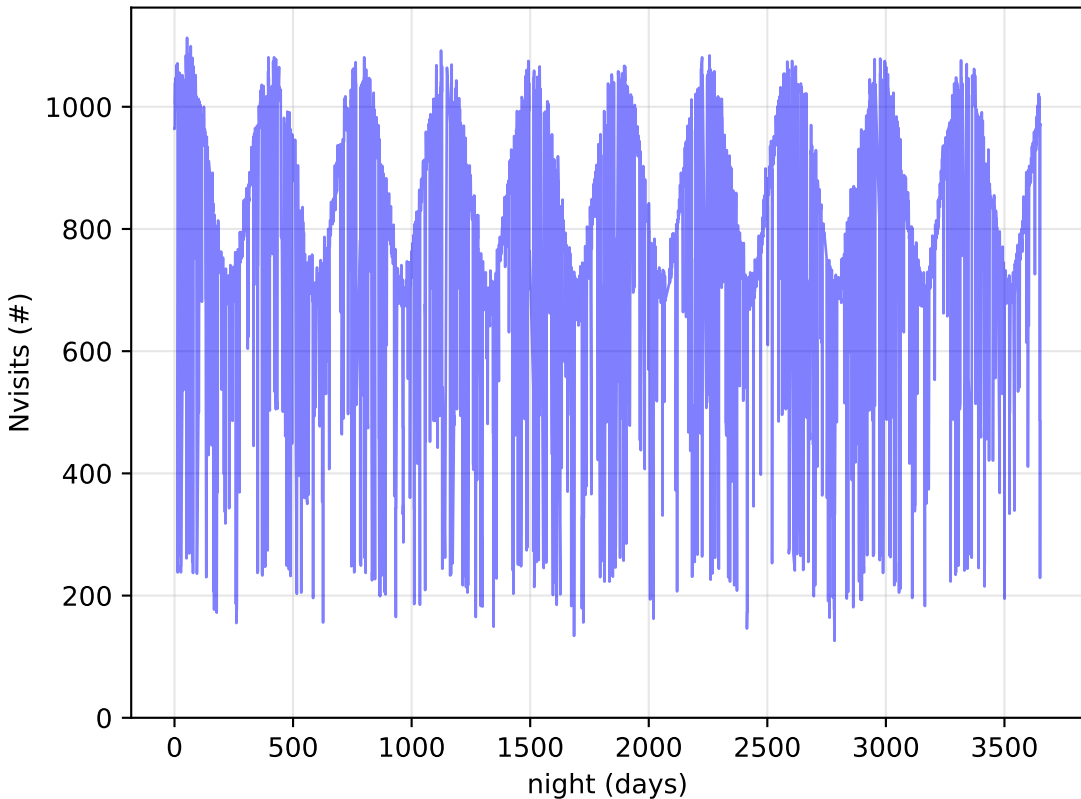
too_elab_2yr_r32_d2_ugrizy_v3.4_10yrs All visits: Nvisits
