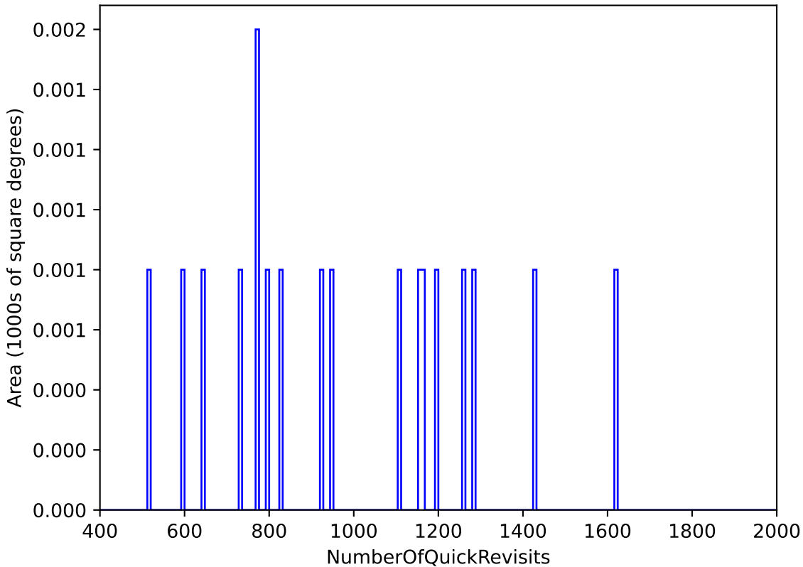
too_elab_2yr_r32_d2_ugrizy_v3.4_10yrs WFD: NumberOfQuickRevisits
