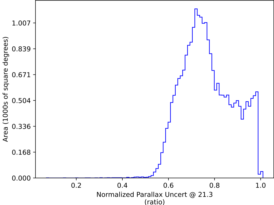
too_elab_2yr_r32_d2_ugrizy_v3.4_10yrs All sky y band only: Normalized Parallax Uncert @ 21.3
