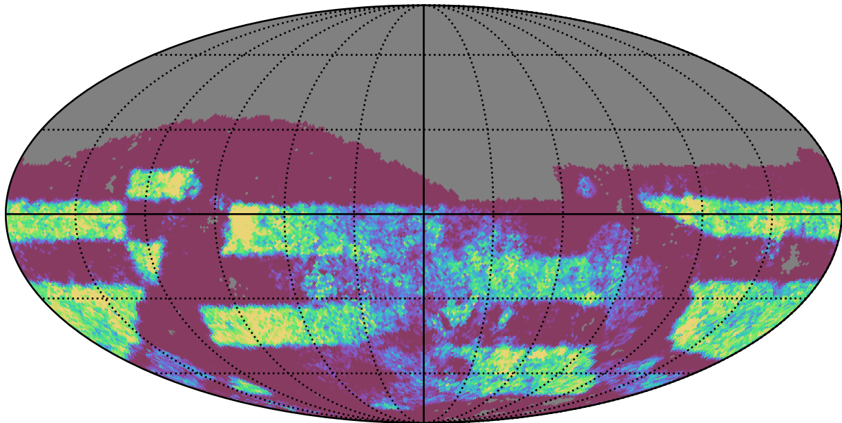
too_elab_2yr_r32_d2_ugrizy_v3.4_10yrs Yr 3-4 z band: NVisits
